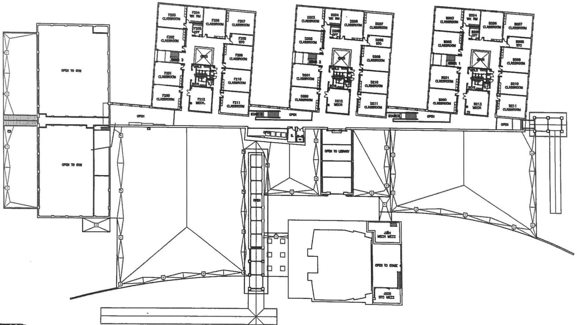
WEST BRIAR MIDDLE SCHOOL LEVEL TWO FIRE EVACUATION PLAN
