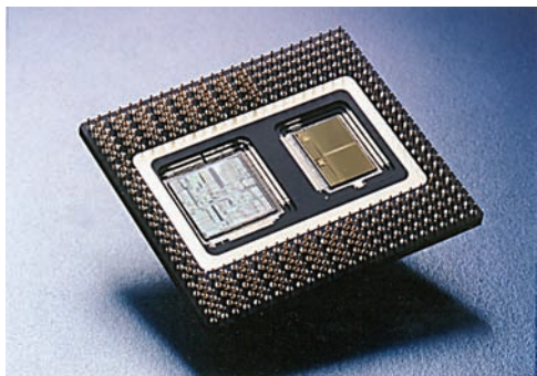
• Figure 5.37 A P6 opened to show separate CPU and L2 cache (photo courtesy of Intel)
