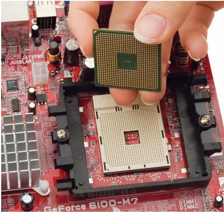
• Figure 5.65 Orienting the CPU
