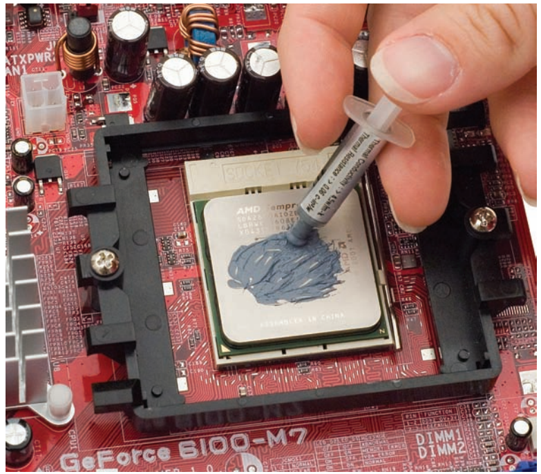
• Figure 5.67 Applying thermal compound
