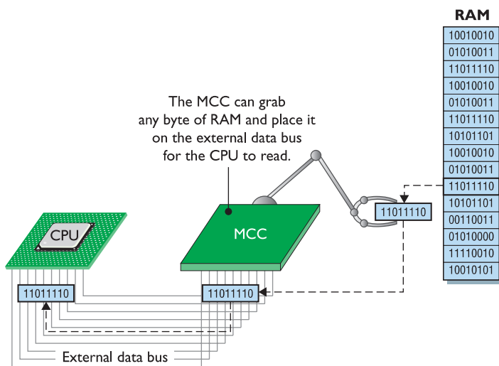
• Figure 5.17 The MCC grabs a byte of RAM.
