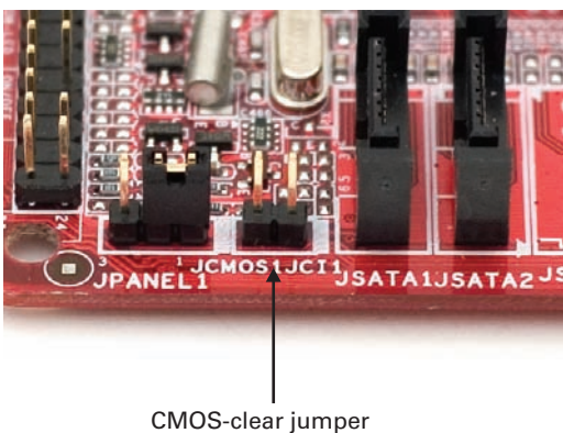
• Figure 5.72 CMOS-clear jumper
