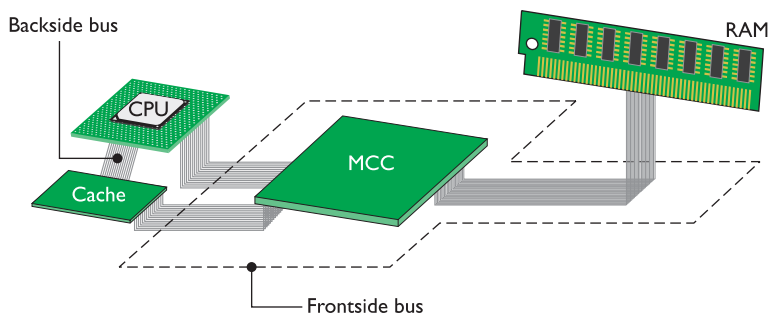
• Figure 5.38 Frontside and backside buses
