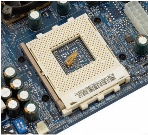
• Figure 5.23 ZIF socket with arm on side
