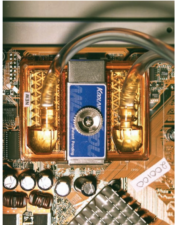
• Figure 5.70 Liquid-cooled CPU
