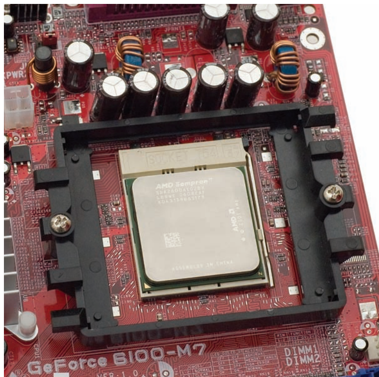
• Figure 5.66 CPU inserted
