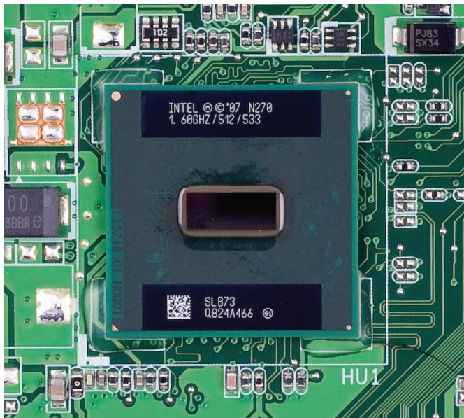
• Figure 5.73 Intel Atom processor
