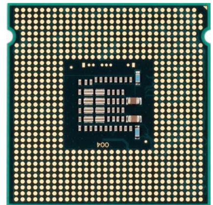
• Figure 5.47 Pentium 4 LGA
