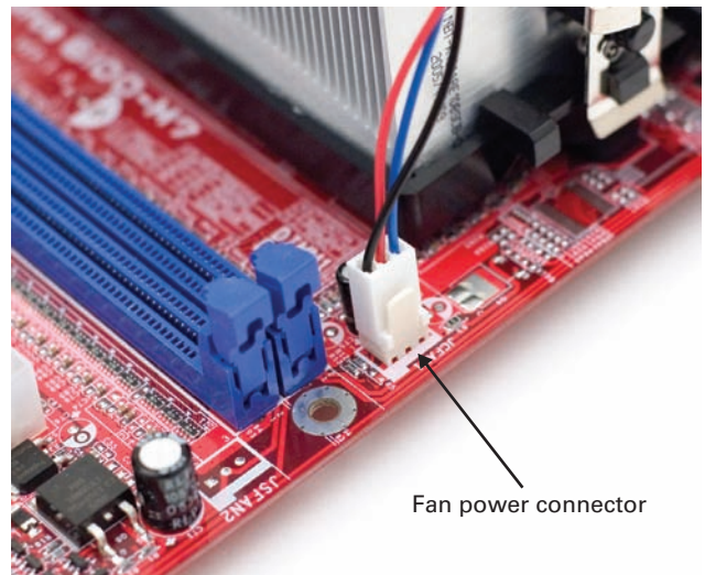
• Figure 5.63 Fan connection
