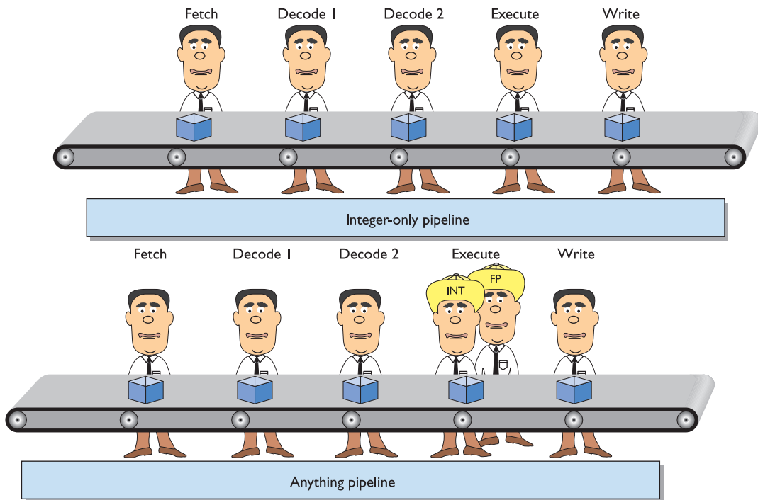
• Figure 5.29 The Pentium dual pipeline
