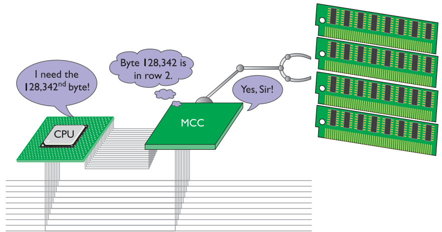
• Figure 6.8 The MCC knows the real location of the DRAM.
