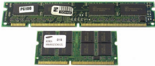
• Figure 6.10 A 168-pin DIMM above a 144-pin SO-DIMM
