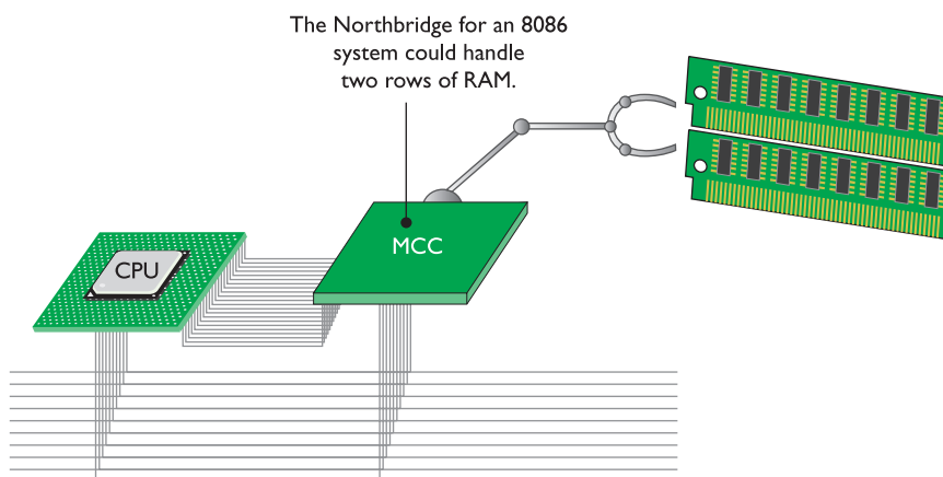
• Figure 6.5 Pumped-up 8086 MCC at work
