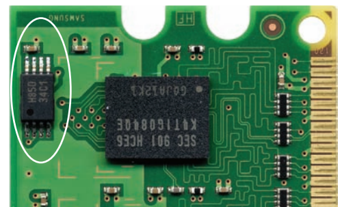
• Figure 6.28 SPD chip on a stick
